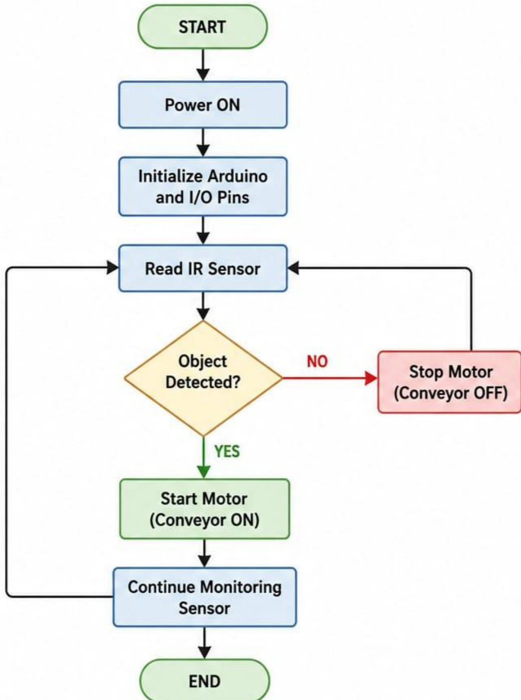
FLOWCHART – SMART CONVEYOR BELT WITH SENSOR
